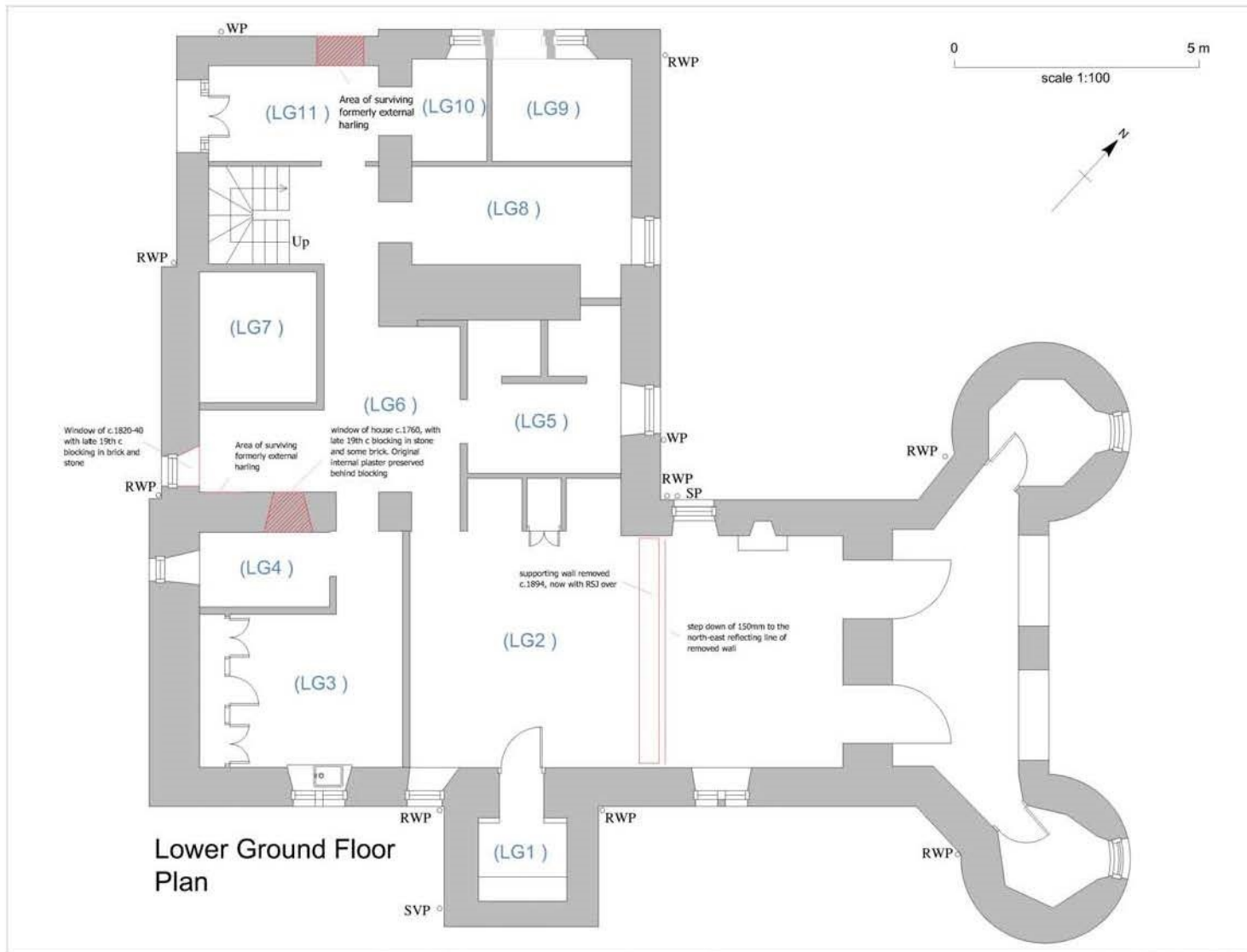
lower ground floor plan with room numbers
