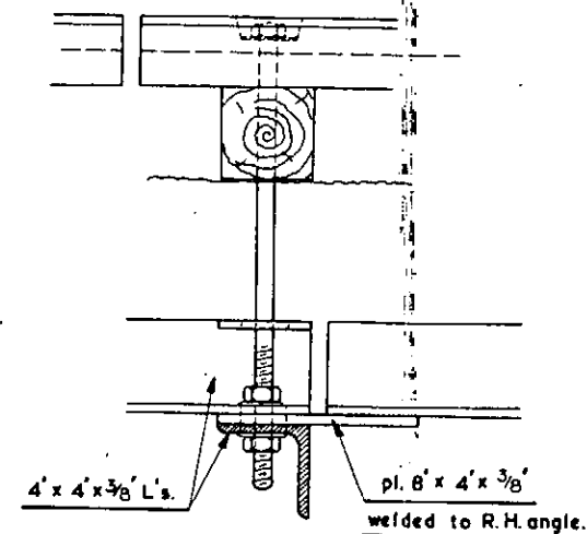
VIEW ON X - X
