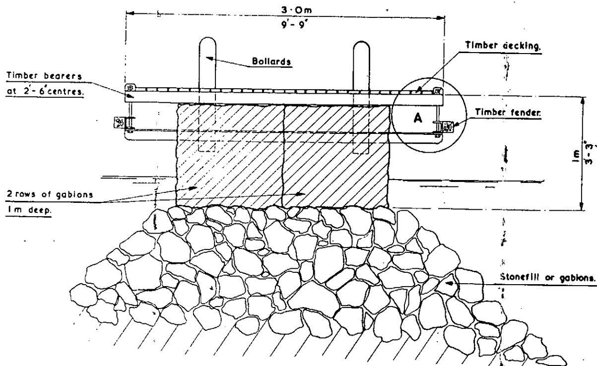
SECTION THROUGH JETTY
