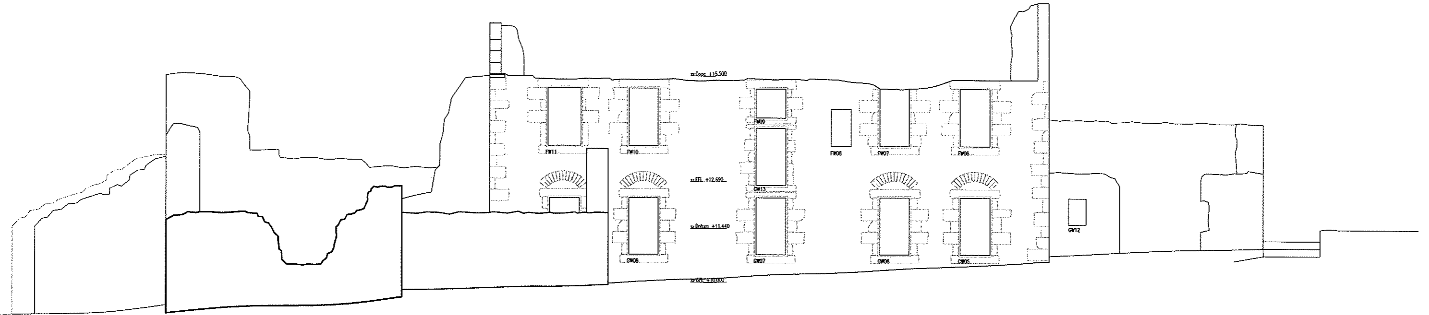
North Elevation
